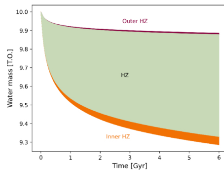
(d) Water loss evolution of Earth orbiting a K-dwarf (HD22049) in Terrestrial Ocean (T.O.) units.
