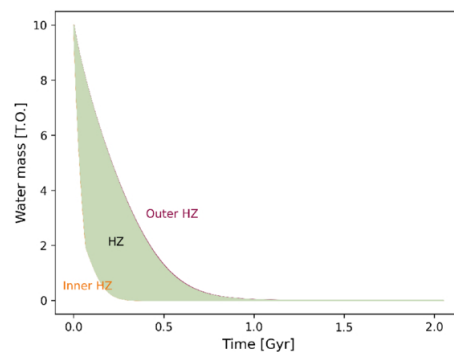
(f) Water loss evolution of Earth orbiting an M-dwarf (TRAPPIST-1) in Terrestrial Ocean (T.O.) units.
