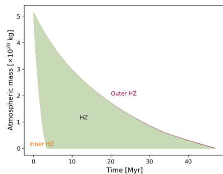
(e) Atmospheric evolution of Earth orbiting an M-dwarf (TRAPPIST-1).
