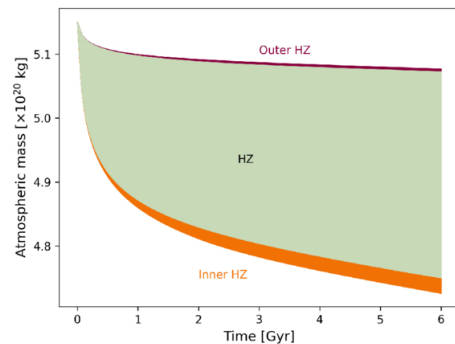
(a) Atmospheric evolution of Earth orbiting a G-dwarf (Sun).
