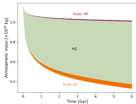
(c) Atmospheric evolution of Earth orbiting a K-dwarf (HD22049).
