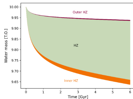
(b) Water loss evolution of Earth orbiting a G-dwarf (Sun) in Terrestrial Ocean (T.O.) units.
