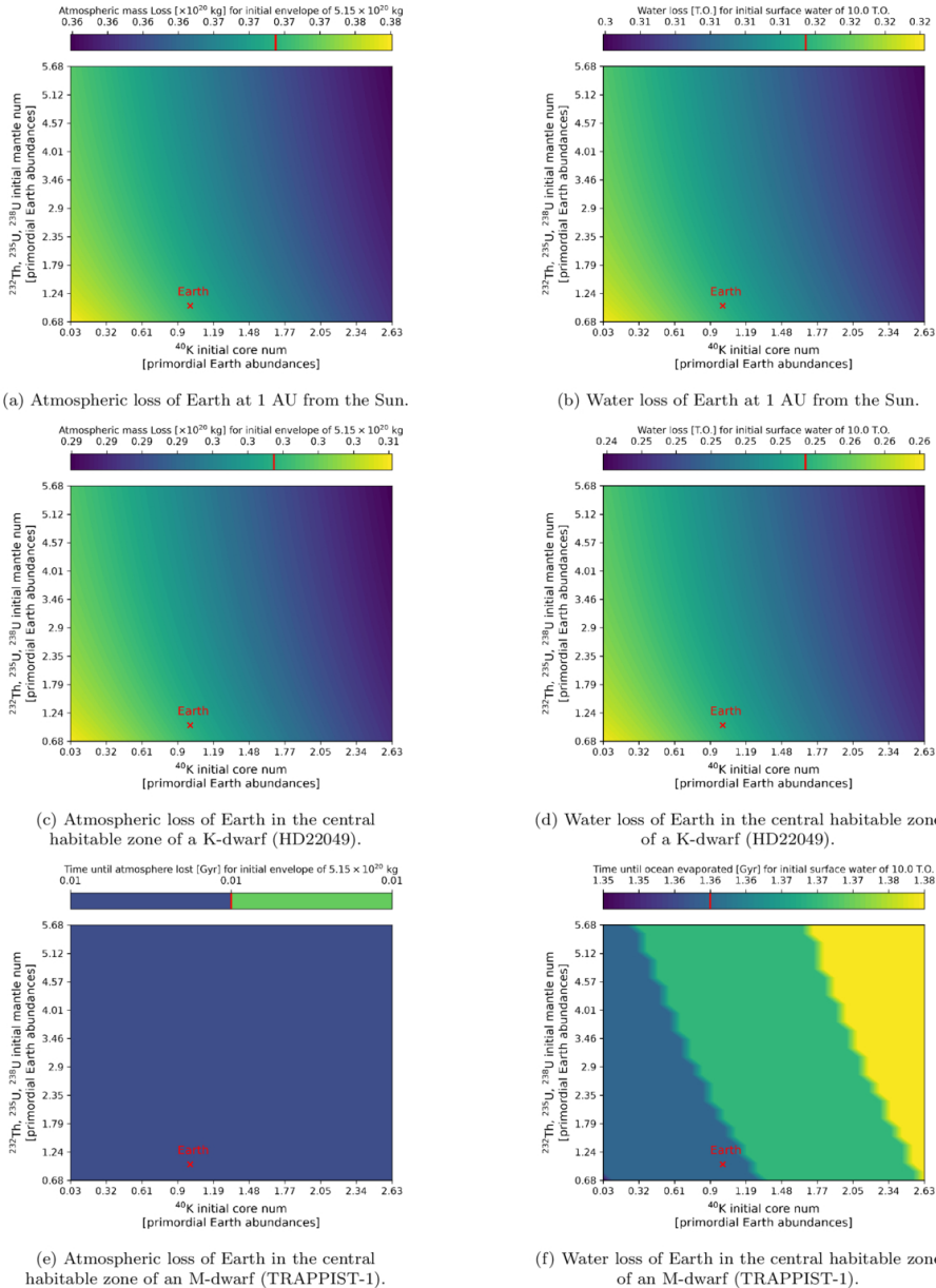
Figure 4. from Nathaniel Tanglin and Juliette Becker 2026 Astrophys. J. 1008 doi:10.3847/1538-4357/ae8f2b https://dx.doi.org/10.3847/1538-4357/ae8f2b © 2026. The Author(s). Published by the American Astronomical Society.
