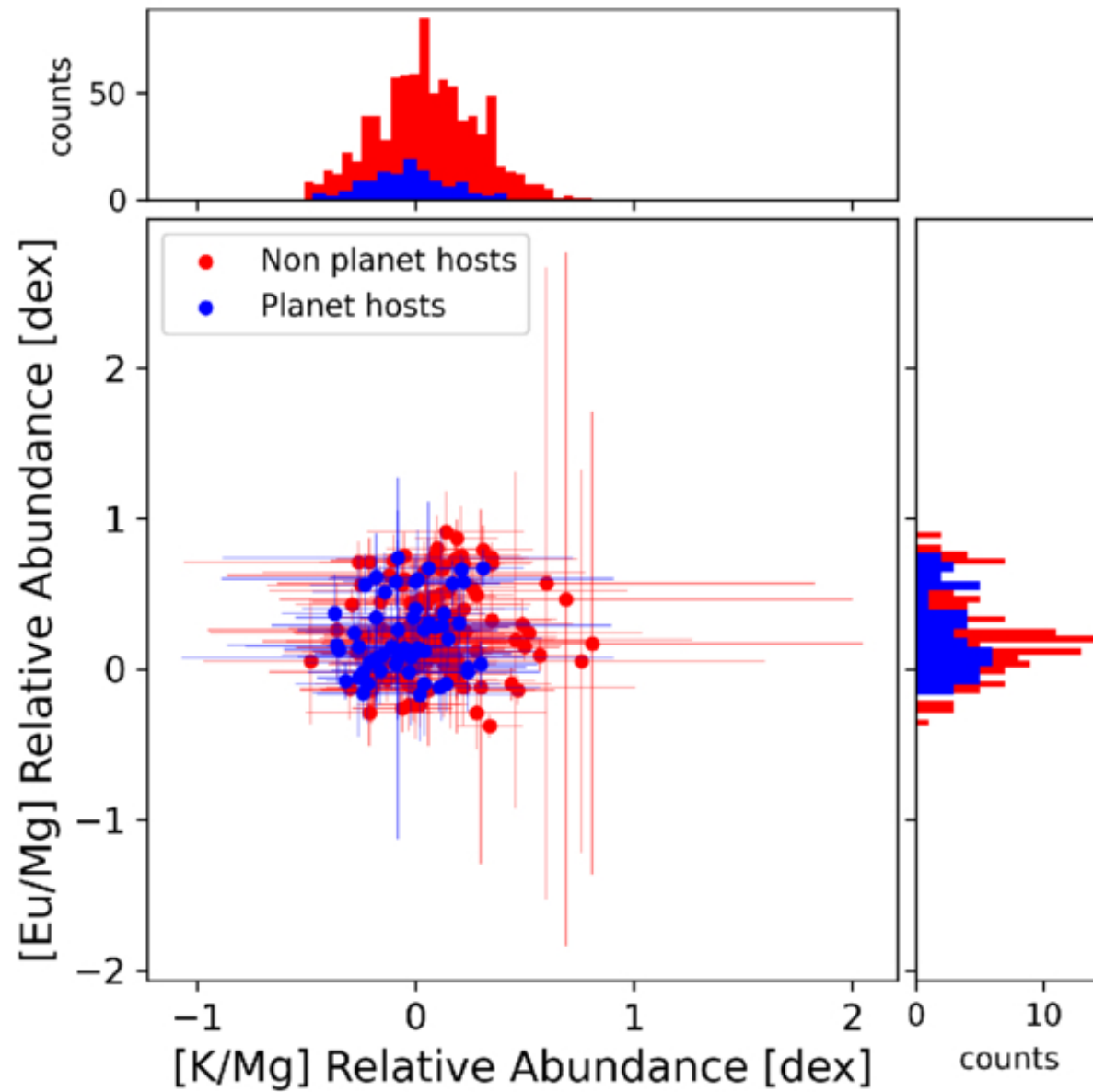
Figure 3. from Nathaniel Tanglin and Juliette Becker 2026 Astrophys. J. 1008 doi:10.3847/1538-4357/ae8f2b https://dx.doi.org/10.3847/1538-4357/ae8f2b © 2026. The Author(s). Published by the American Astronomical Society.
