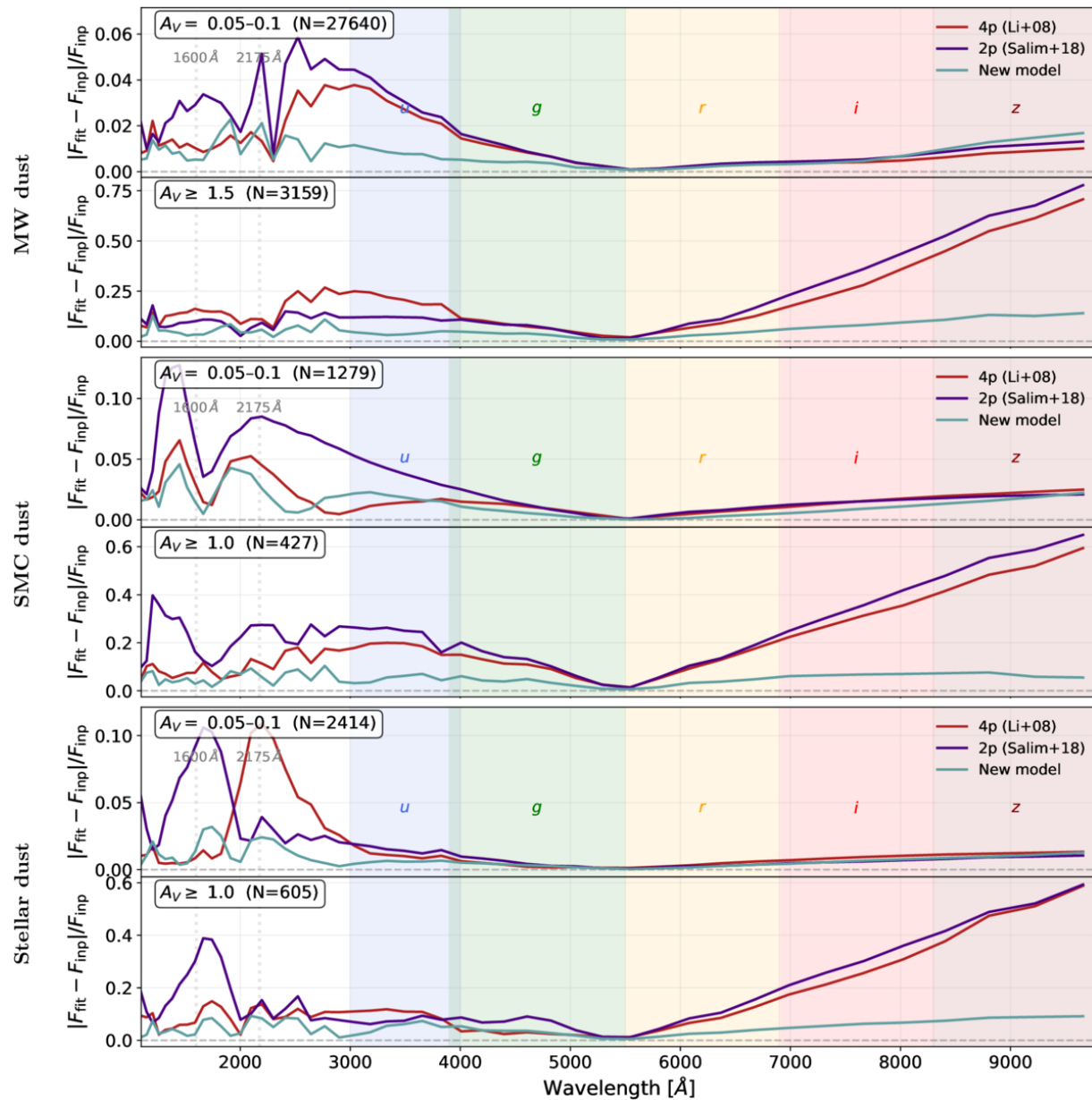
Figure 8. from Laura Sommovigo et al 2026 Astrophys. J. 1008 doi:10.3847/1538-4357/ae8e78 https://dx.doi.org/10.3847/1538-4357/ae8e78 © 2026. The Author(s). Published by the American Astronomical Society.
