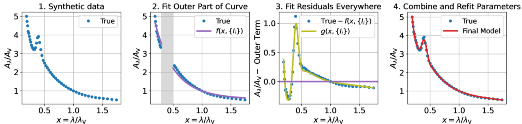
Figure 3. from Laura Sommovigo et al 2026 Astrophys. J. 1008 doi:10.3847/1538-4357/ae8e78 https://dx.doi.org/10.3847/1538-4357/ae8e78 © 2026. The Author(s). Published by the American Astronomical Society.
