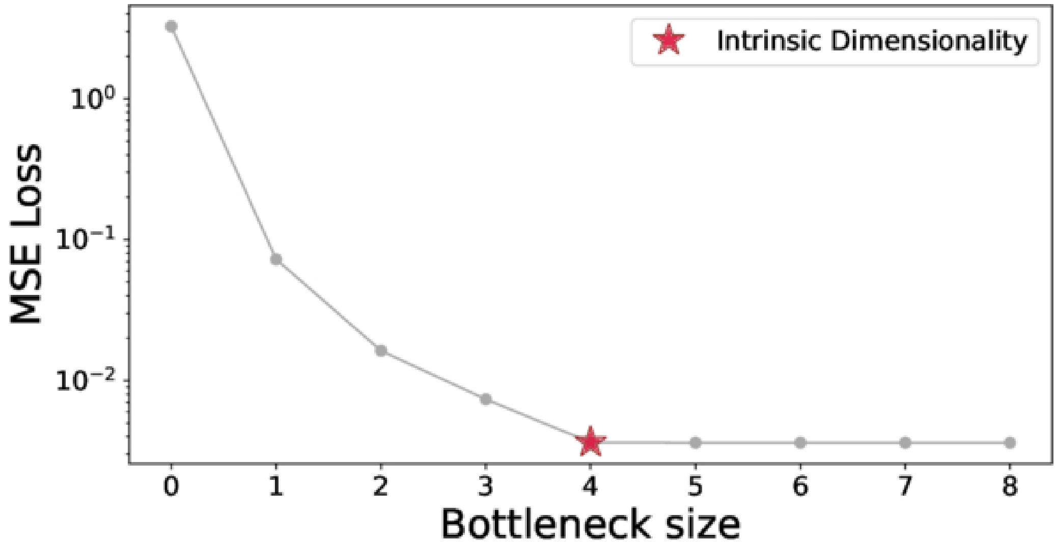
Figure 2. from Laura Sommovigo et al 2026 Astrophys. J. 1008 doi:10.3847/1538-4357/ae8e78 https://dx.doi.org/10.3847/1538-4357/ae8e78 © 2026. The Author(s). Published by the American Astronomical Society.
