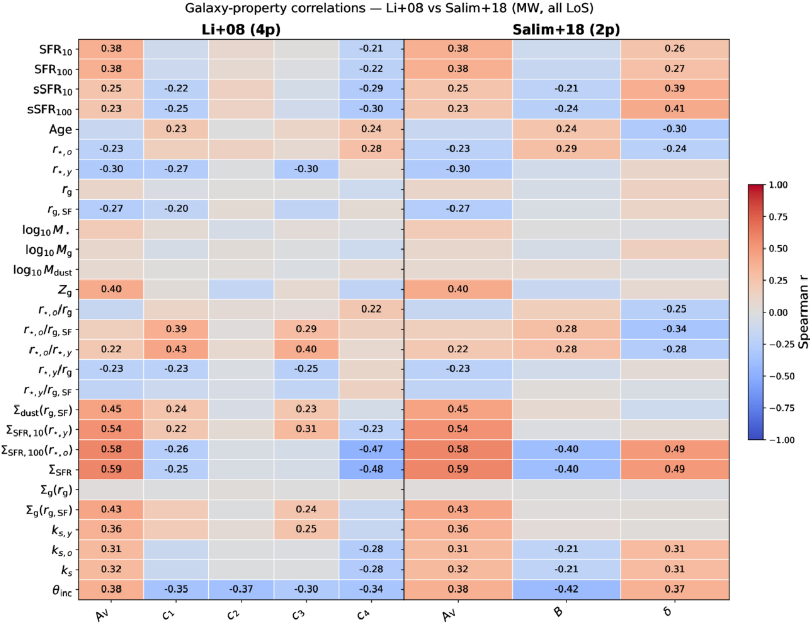
Figure A1. from Laura Sommovigo et al 2026 Astrophys. J. 1008 doi:10.3847/1538-4357/ae8e78 https://dx.doi.org/10.3847/1538-4357/ae8e78 © 2026. The Author(s). Published by the American Astronomical Society.
