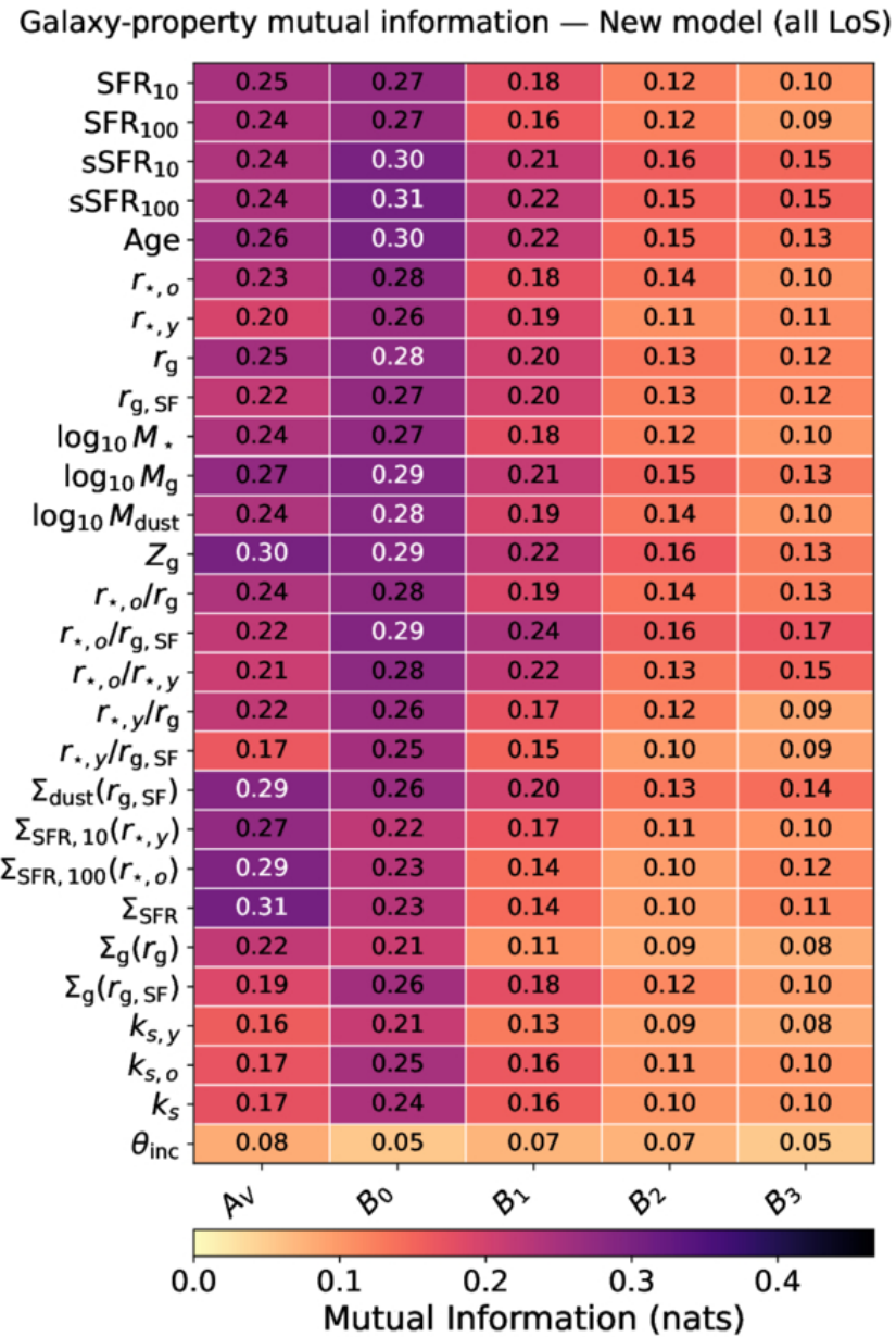
Figure 13. from Laura Sommovigo et al 2026 Astrophys. J. 1008 doi:10.3847/1538-4357/ae8e78 https://dx.doi.org/10.3847/1538-4357/ae8e78 © 2026. The Author(s). Published by the American Astronomical Society.
