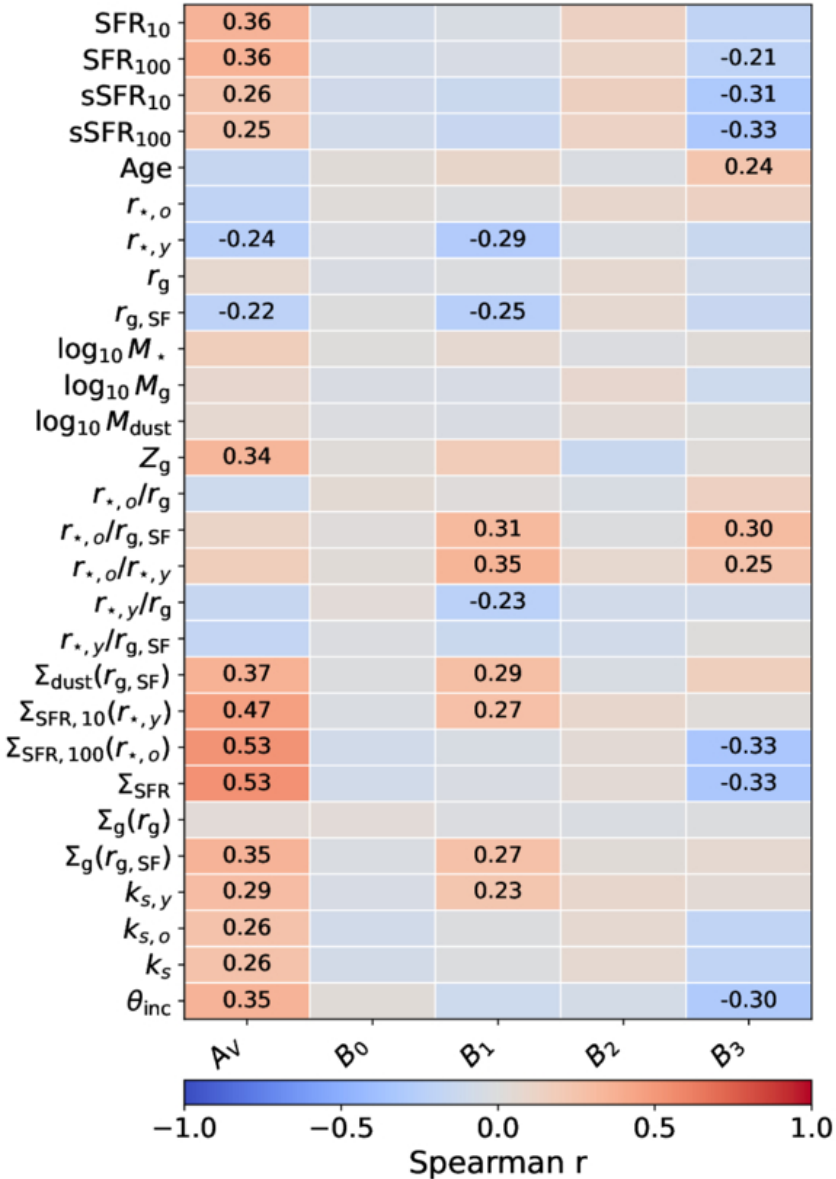
Figure 12. from Laura Sommovigo et al 2026 Astrophys. J. 1008 doi:10.3847/1538-4357/ae8e78 https://dx.doi.org/10.3847/1538-4357/ae8e78 © 2026. The Author(s). Published by the American Astronomical Society. Galaxy-property Spearman correlations — New model (all LoS)
