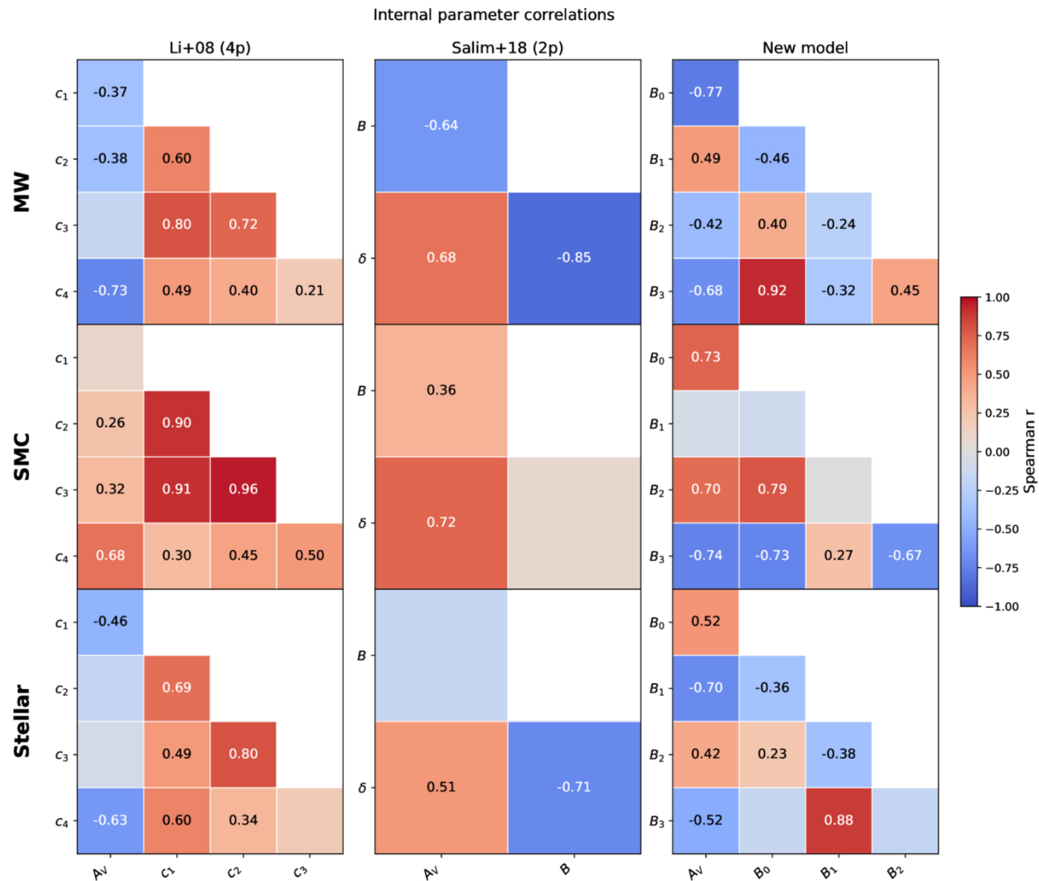
Figure 11. from Laura Sommovigo et al 2026 Astrophys. J. 1008 doi:10.3847/1538-4357/ae8e78 https://dx.doi.org/10.3847/1538-4357/ae8e78 © 2026. The Author(s). Published by the American Astronomical Society.
