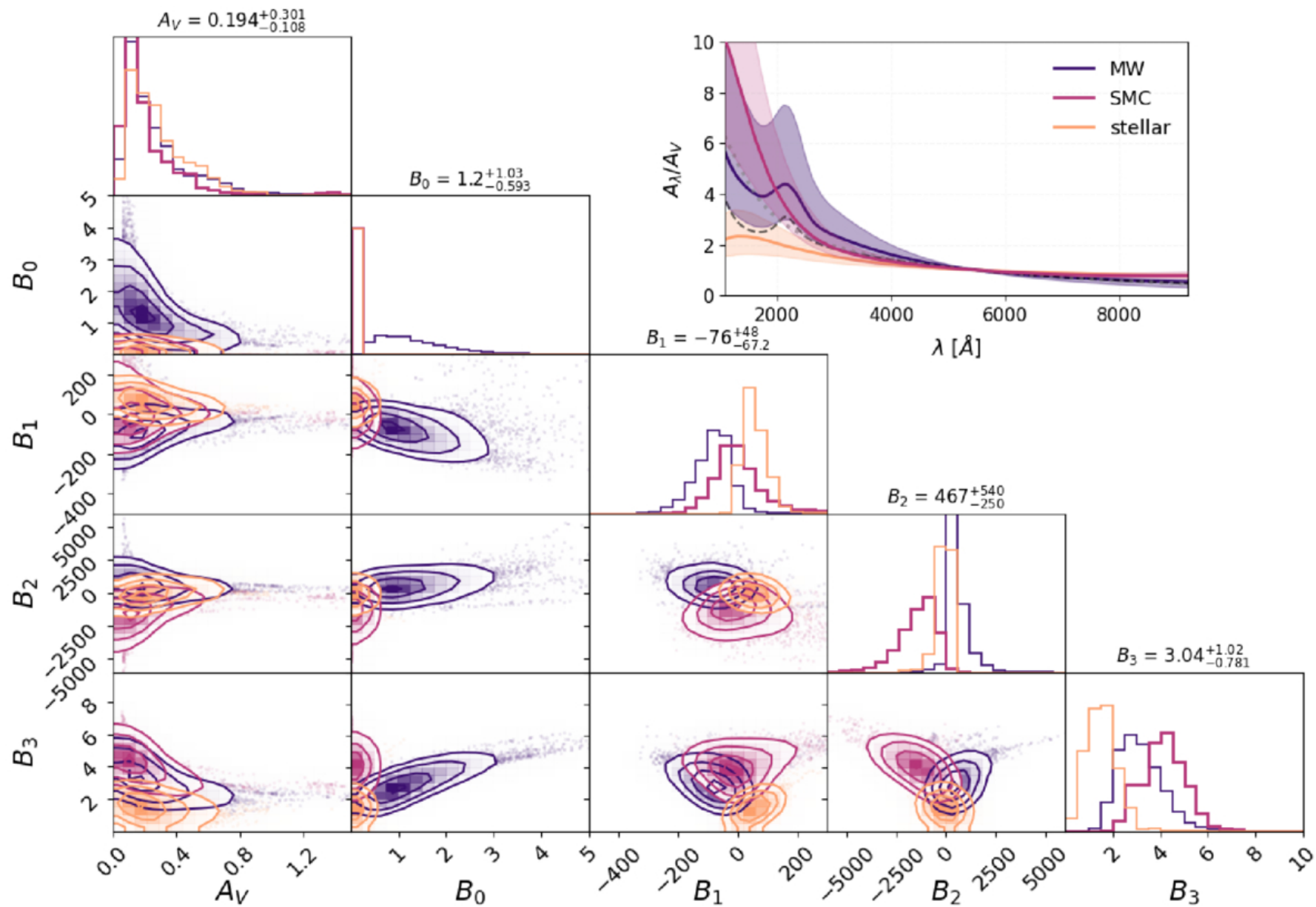
Figure 10. from Laura Sommovigo et al 2026 Astrophys. J. 1008 doi:10.3847/1538-4357/ae8e78 https://dx.doi.org/10.3847/1538-4357/ae8e78 © 2026. The Author(s). Published by the American Astronomical Society.
