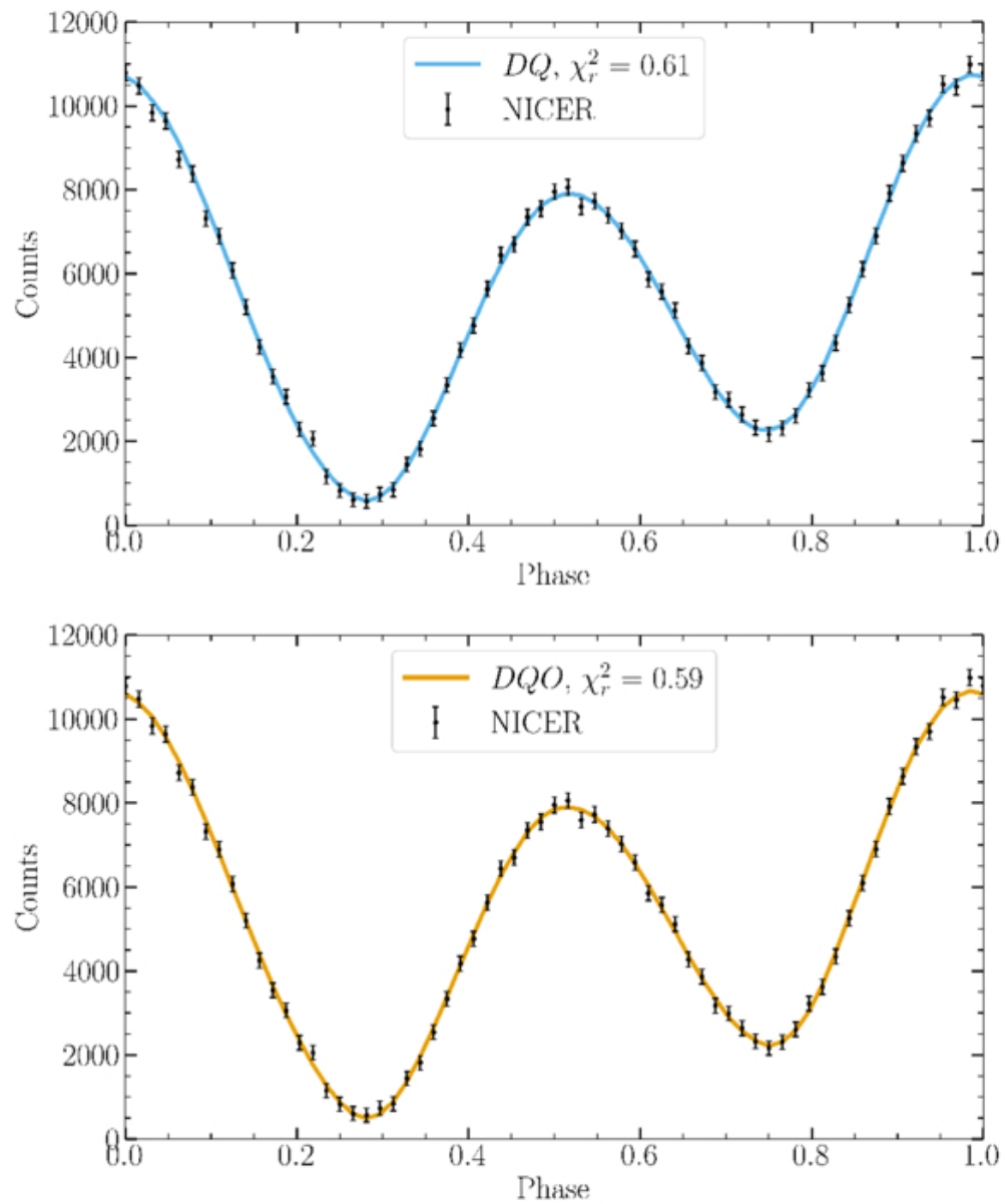
Figure 8. from Anu Kundu et al 2026 Astrophys. J. 1008 doi:10.3847/1538-4357/ae8e6f https://dx.doi.org/10.3847/1538-4357/ae8e6f © 2026. The Author(s). Published by the American Astronomical Society.
