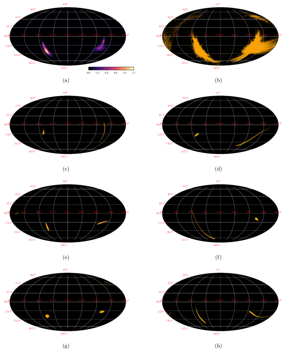
Figure 7. from Anu Kundu et al 2026 Astrophys. J. 1008 doi:10.3847/1538-4357/ae8e6f https://dx.doi.org/10.3847/1538-4357/ae8e6f © 2026. The Author(s). Published by the American Astronomical Society.
