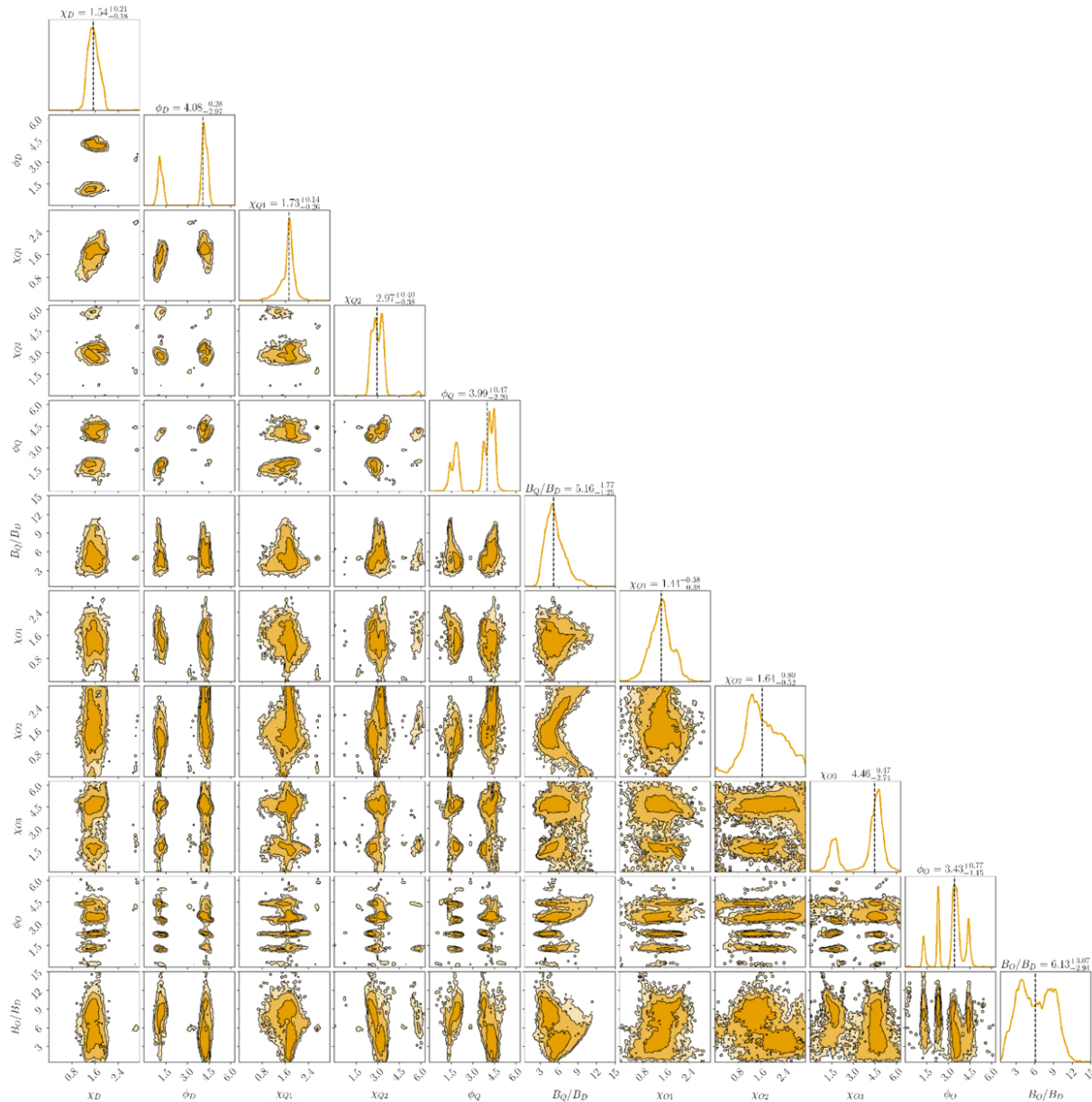
Figure 4. from Anu Kundu et al 2026 Astrophys. J. 1008 doi:10.3847/1538-4357/ae8e6f https://dx.doi.org/10.3847/1538-4357/ae8e6f © 2026. The Author(s). Published by the American Astronomical Society.
