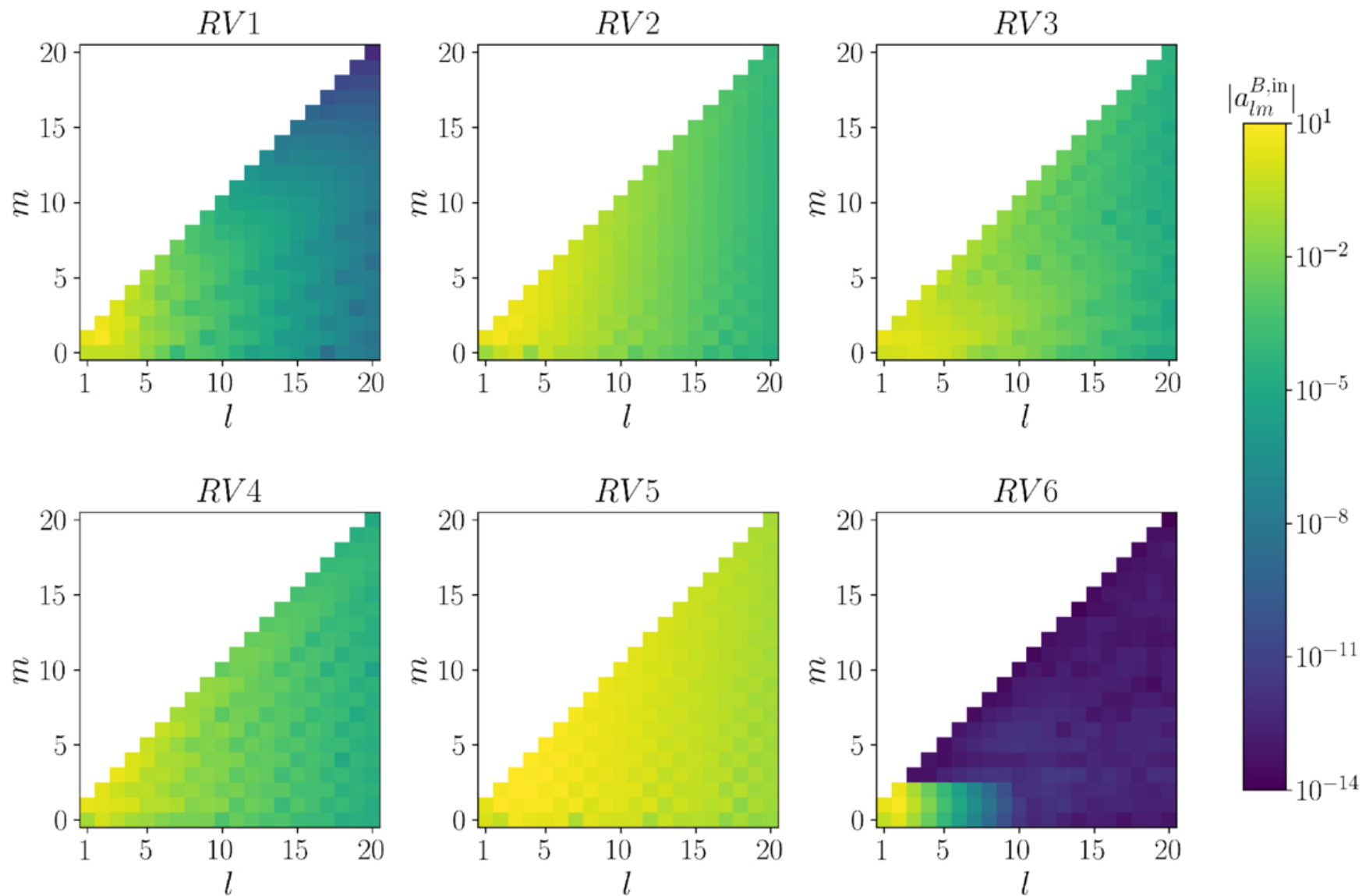
Figure 1. from Anu Kundu et al 2026 Astrophys. J. 1008 doi:10.3847/1538-4357/ae8e6f https://dx.doi.org/10.3847/1538-4357/ae8e6f © 2026. The Author(s). Published by the American Astronomical Society.
