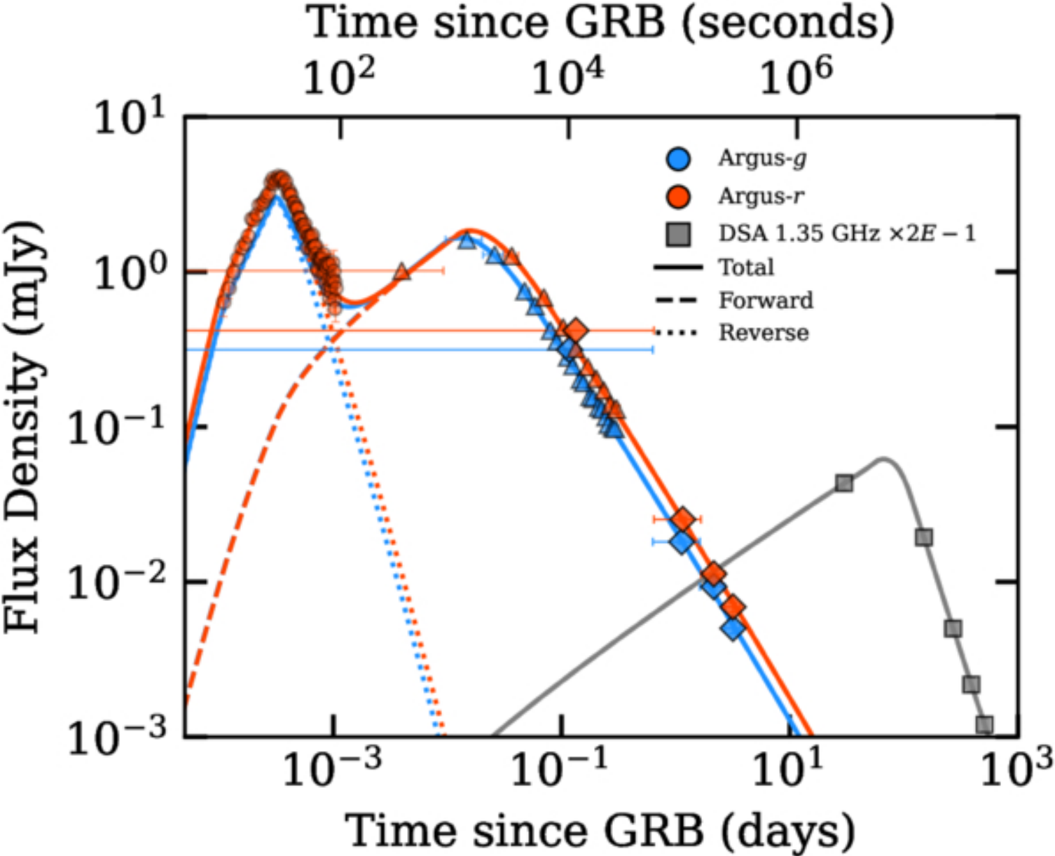
Figure 8. from James Freeburn et al 2026 Astrophys. J. 1007 doi:10.3847/1538-4357/ae8e6b https://dx.doi.org/10.3847/1538-4357/ae8e6b © 2026. The Author(s). Published by the American Astronomical Society.
