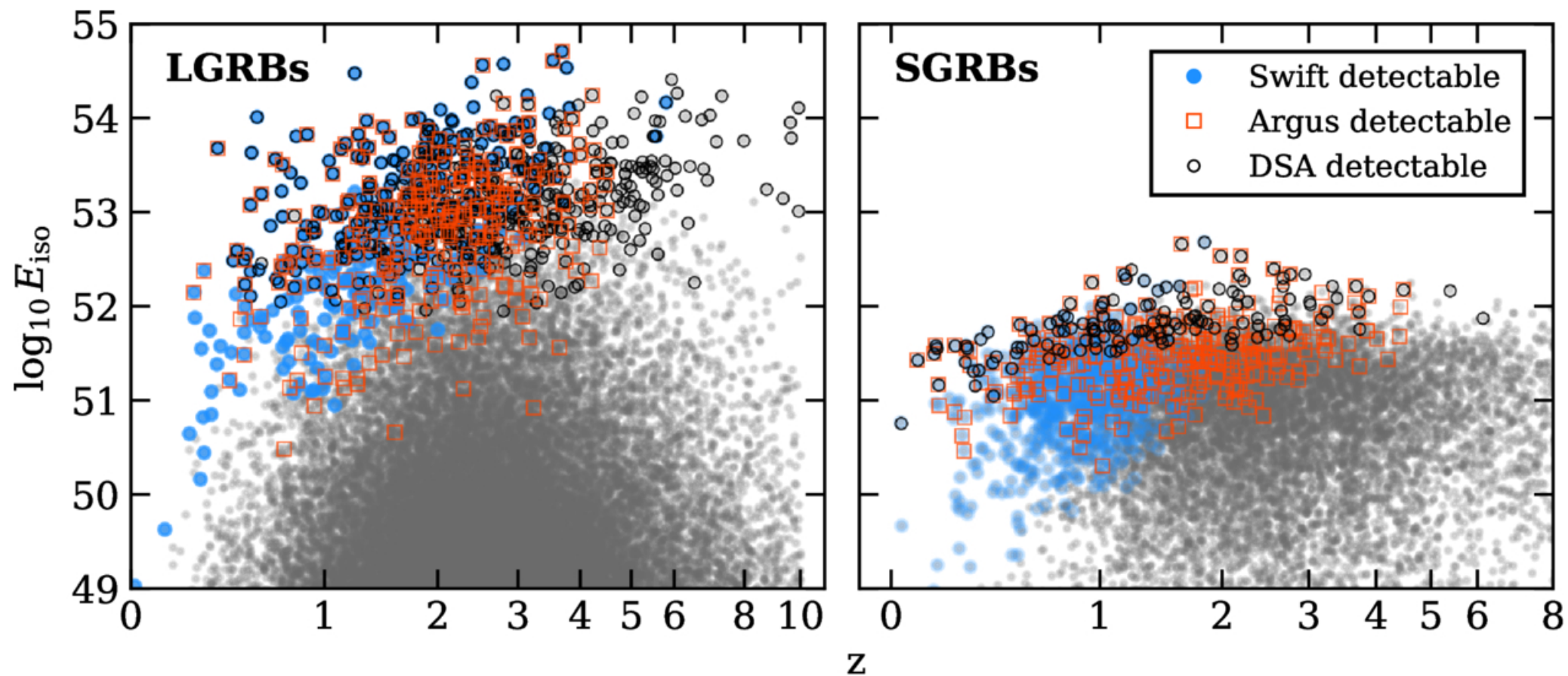
Figure 5. from James Freeburn et al 2026 Astrophys. J. 1007 doi:10.3847/1538-4357/ae8e6b https://dx.doi.org/10.3847/1538-4357/ae8e6b © 2026. The Author(s). Published by the American Astronomical Society.
