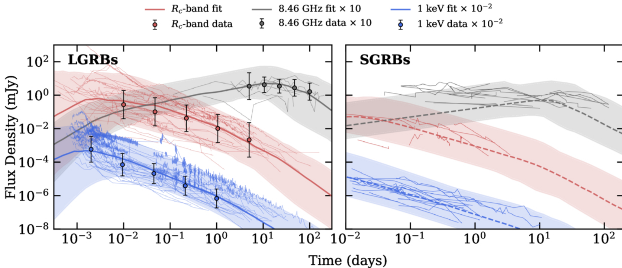
Figure 2. from James Freeburn et al 2026 Astrophys. J. 1007 doi:10.3847/1538-4357/ae8e6b https://dx.doi.org/10.3847/1538-4357/ae8e6b © 2026. The Author(s). Published by the American Astronomical Society.
