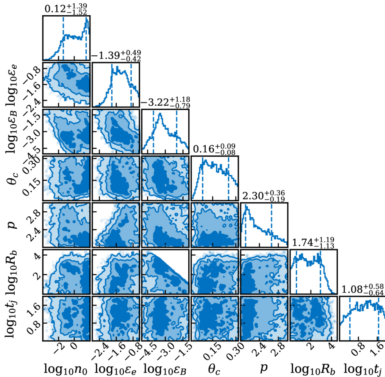
Figure 1. from James Freeburn et al 2026 Astrophys. J. 1007 doi:10.3847/1538-4357/ae8e6b https://dx.doi.org/10.3847/1538-4357/ae8e6b © 2026. The Author(s). Published by the American Astronomical Society.
