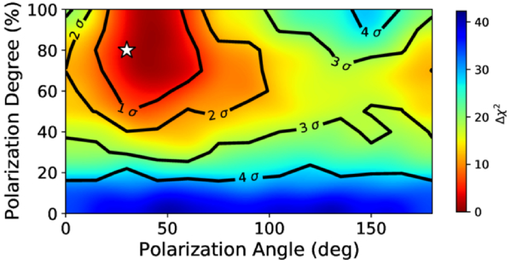
Figure 5. from P. Veres et al 2026 Astrophys. J. 1008 doi:10.3847/1538-4357/ae8dbf https://dx.doi.org/10.3847/1538-4357/ae8dbf © 2026. The Author(s). Published by the American Astronomical Society.
