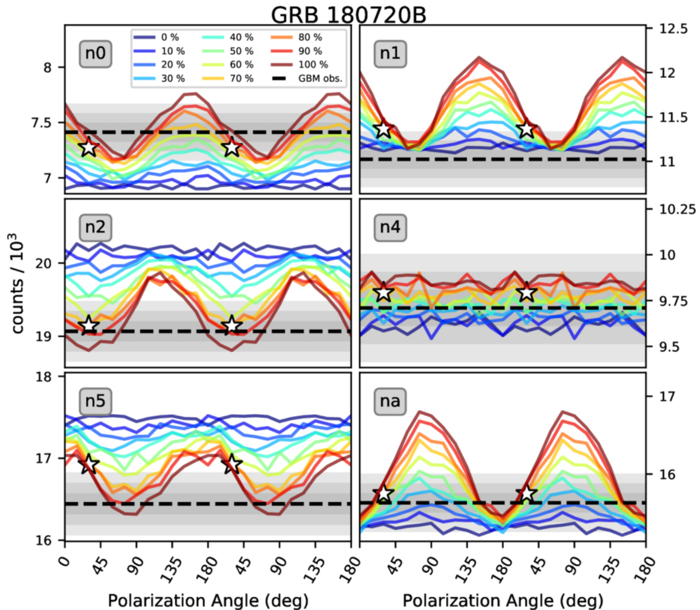
Figure 4. from P. Veres et al 2026 Astrophys. J. 1008 doi:10.3847/1538-4357/ae8dbf https://dx.doi.org/10.3847/1538-4357/ae8dbf © 2026. The Author(s). Published by the American Astronomical Society.
