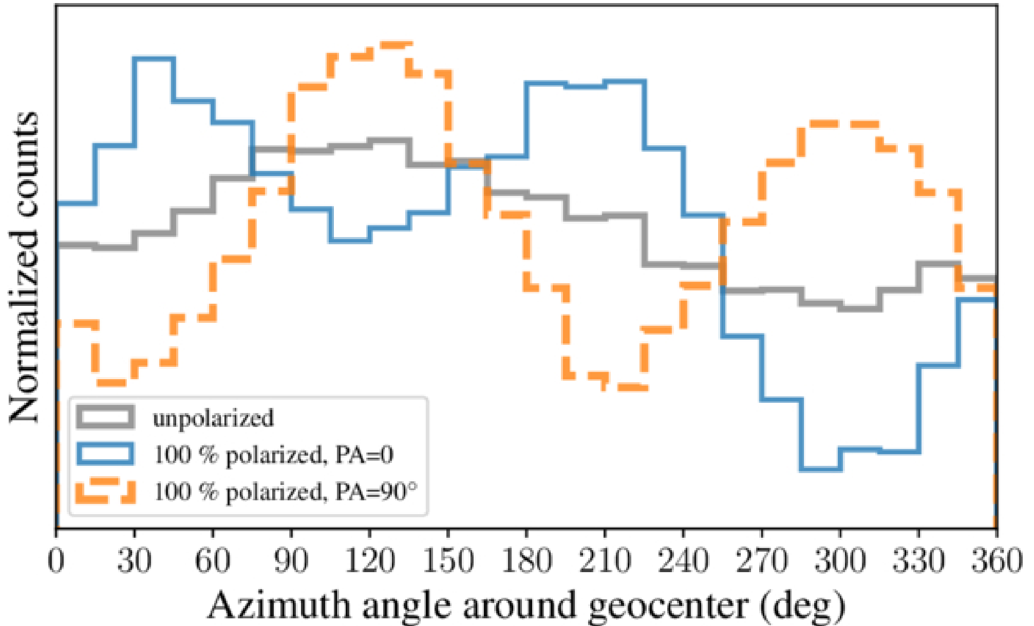
Figure 3. from P. Veres et al 2026 Astrophys. J. 1008 doi:10.3847/1538-4357/ae8dbf https://dx.doi.org/10.3847/1538-4357/ae8dbf © 2026. The Author(s). Published by the American Astronomical Society.
