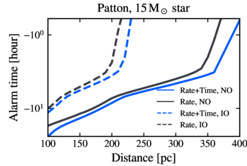
(f) Combined, Patton model signal
