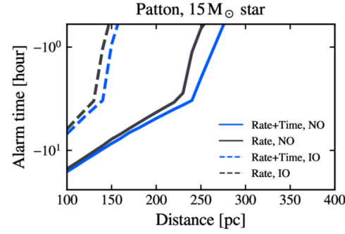
(b) KamLAND, Patton model signal
