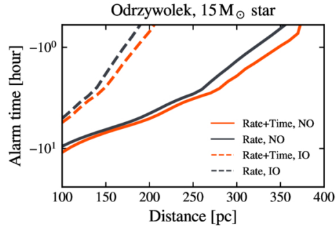
(c) SK, Odrzywolek model signal
