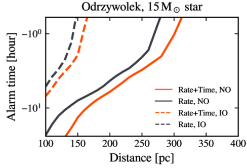
(a) KamLAND, Odrzywolek model signal
