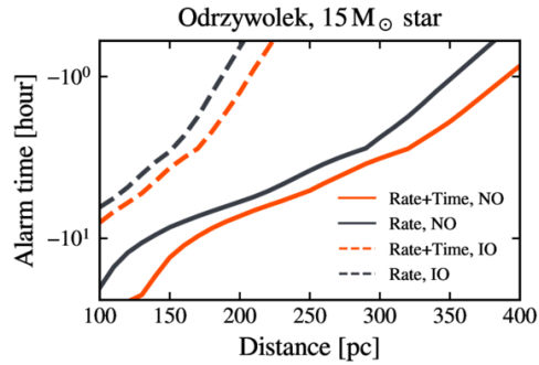
(e) Combined, Odrzywolek model signal
