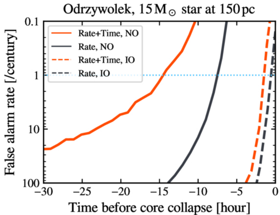
Figure 3. from K. Saito et al 2026 Astrophys. J. 1008 doi:10.3847/1538-4357/ae8da5 https://dx.doi.org/10.3847/1538-4357/ae8da5 © 2026. The Author(s). Published by the American Astronomical Society.
