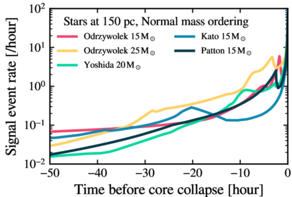
Figure 2. from K. Saito et al 2026 Astrophys. J. 1008 doi:10.3847/1538-4357/ae8da5 https://dx.doi.org/10.3847/1538-4357/ae8da5 © 2026. The Author(s). Published by the American Astronomical Society.
