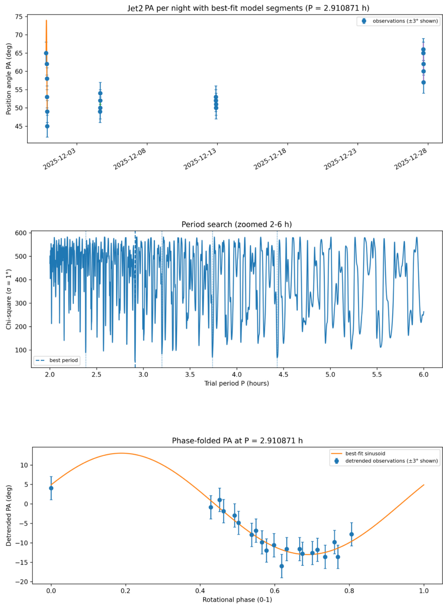
Figure 8. from Toni Scarmato and Abraham Loeb 2026 Astrophys. J. 1009 doi:10.3847/1538-4357/ae8a4a https://dx.doi.org/10.3847/1538-4357/ae8a4a © 2026. The Author(s). Published by the American Astronomical Society.
