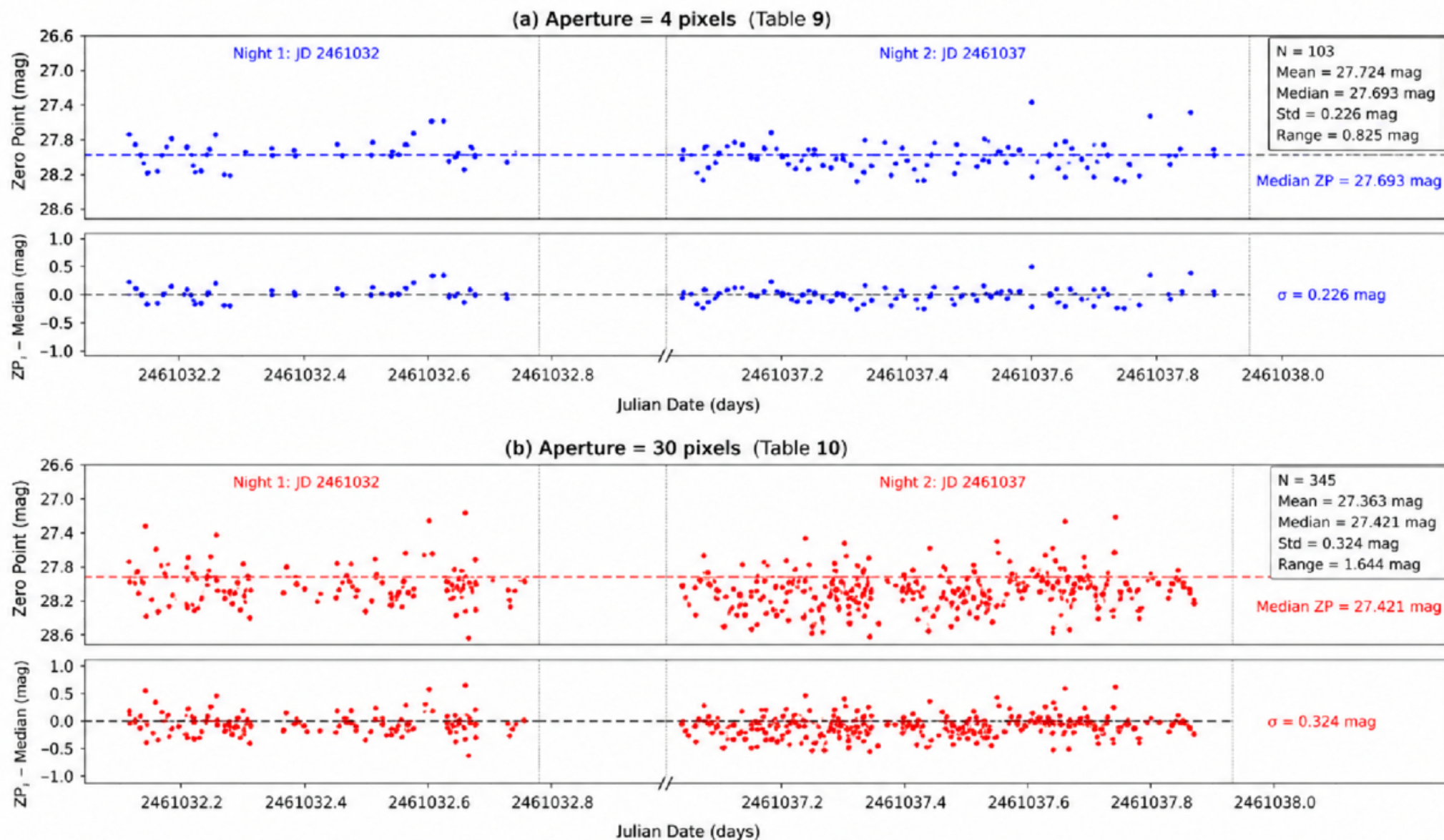
Figure 4. from Toni Scarmato and Abraham Loeb 2026 Astrophys. J. 1009 doi:10.3847/1538-4357/ae8a4a https://dx.doi.org/10.3847/1538-4357/ae8a4a © 2026. The Author(s). Published by the American Astronomical Society.
