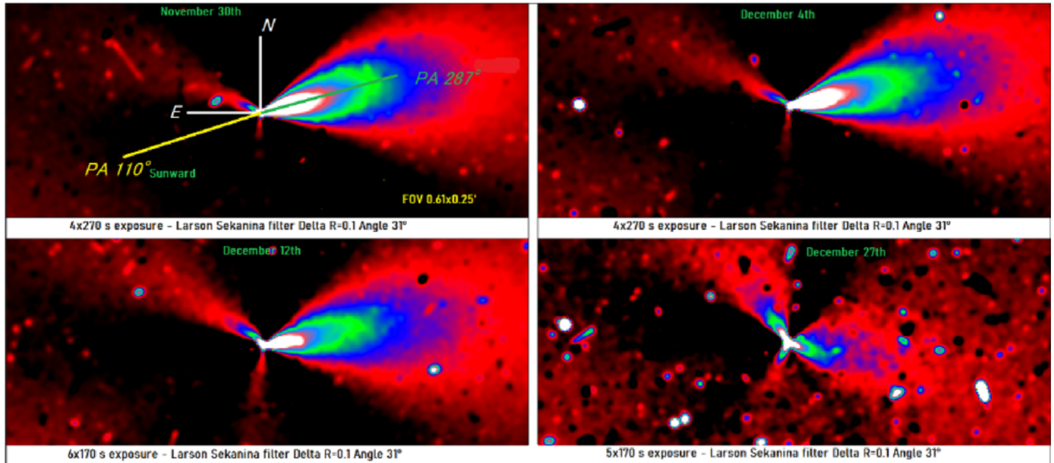
Figure 2. from Toni Scarmato and Abraham Loeb 2026 Astrophys. J. 1009 doi:10.3847/1538-4357/ae8a4a https://dx.doi.org/10.3847/1538-4357/ae8a4a © 2026. The Author(s). Published by the American Astronomical Society.
