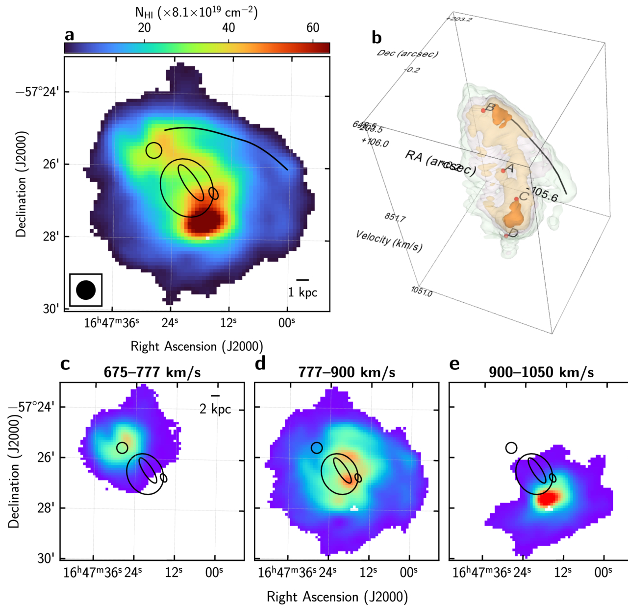
Figure 2. from R. Guimarães Silva et al 2026 Astrophys. J. 1008 doi:10.3847/1538-4357/ae89b7 https://dx.doi.org/10.3847/1538-4357/ae89b7 © 2026. The Author(s). Published by the American Astronomical Society.
