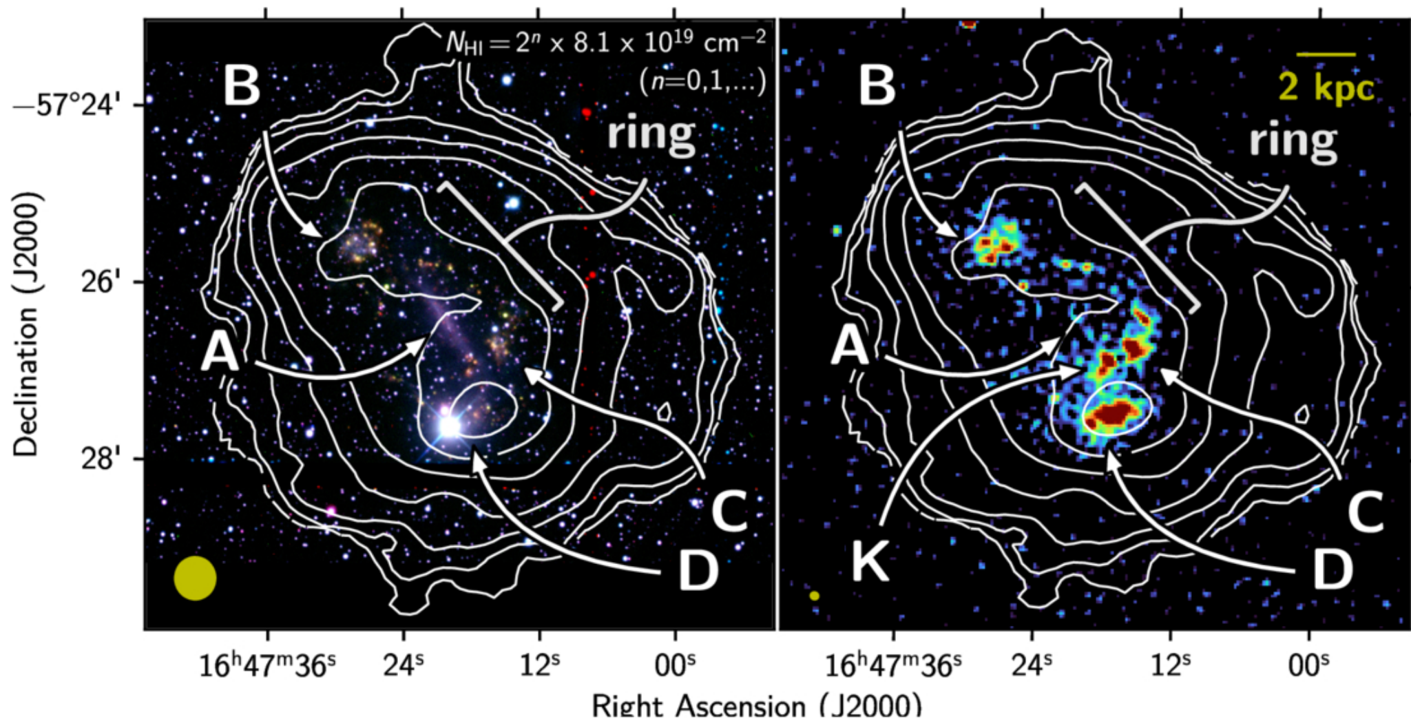
Figure 1. from R. Guimarães Silva et al 2026 Astrophys. J. 1008 doi:10.3847/1538-4357/ae89b7 https://dx.doi.org/10.3847/1538-4357/ae89b7 © 2026. The Author(s). Published by the American Astronomical Society.
