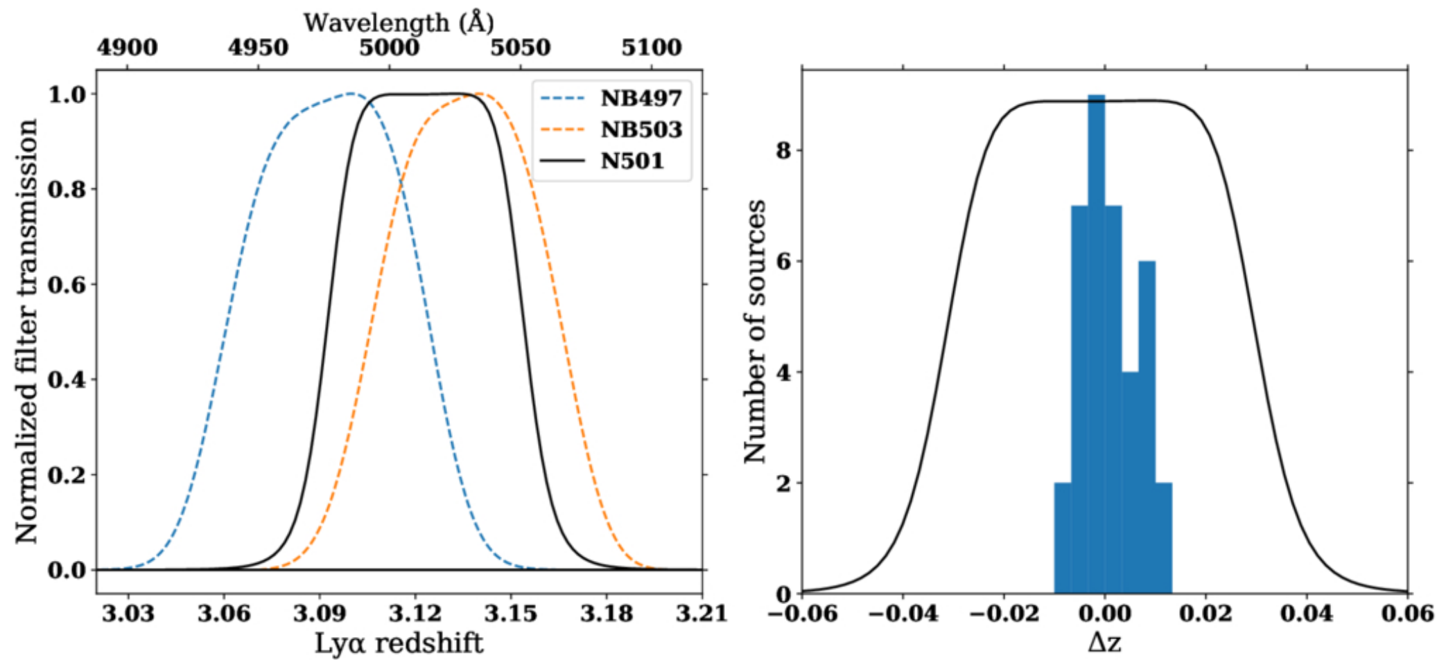
Figure 2. from Ashley Ortiz et al 2026 Astrophys. J. 1008 doi:10.3847/1538-4357/ae899d https://dx.doi.org/10.3847/1538-4357/ae899d © 2026. The Author(s). Published by the American Astronomical Society.
