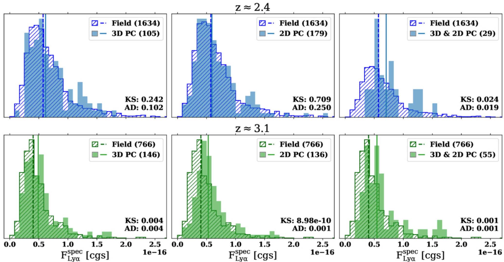
Figure 10. from Ashley Ortiz et al 2026 Astrophys. J. 1008 doi:10.3847/1538-4357/ae899d https://dx.doi.org/10.3847/1538-4357/ae899d © 2026. The Author(s). Published by the American Astronomical Society.
