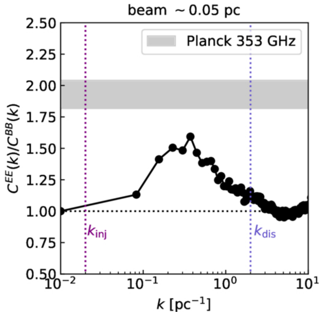
Figure 9. from Yue Hu et al 2026 Astrophys. J. 1007 doi:10.3847/1538-4357/ae8998 https://dx.doi.org/10.3847/1538-4357/ae8998 © 2026. The Author(s). Published by the American Astronomical Society.
