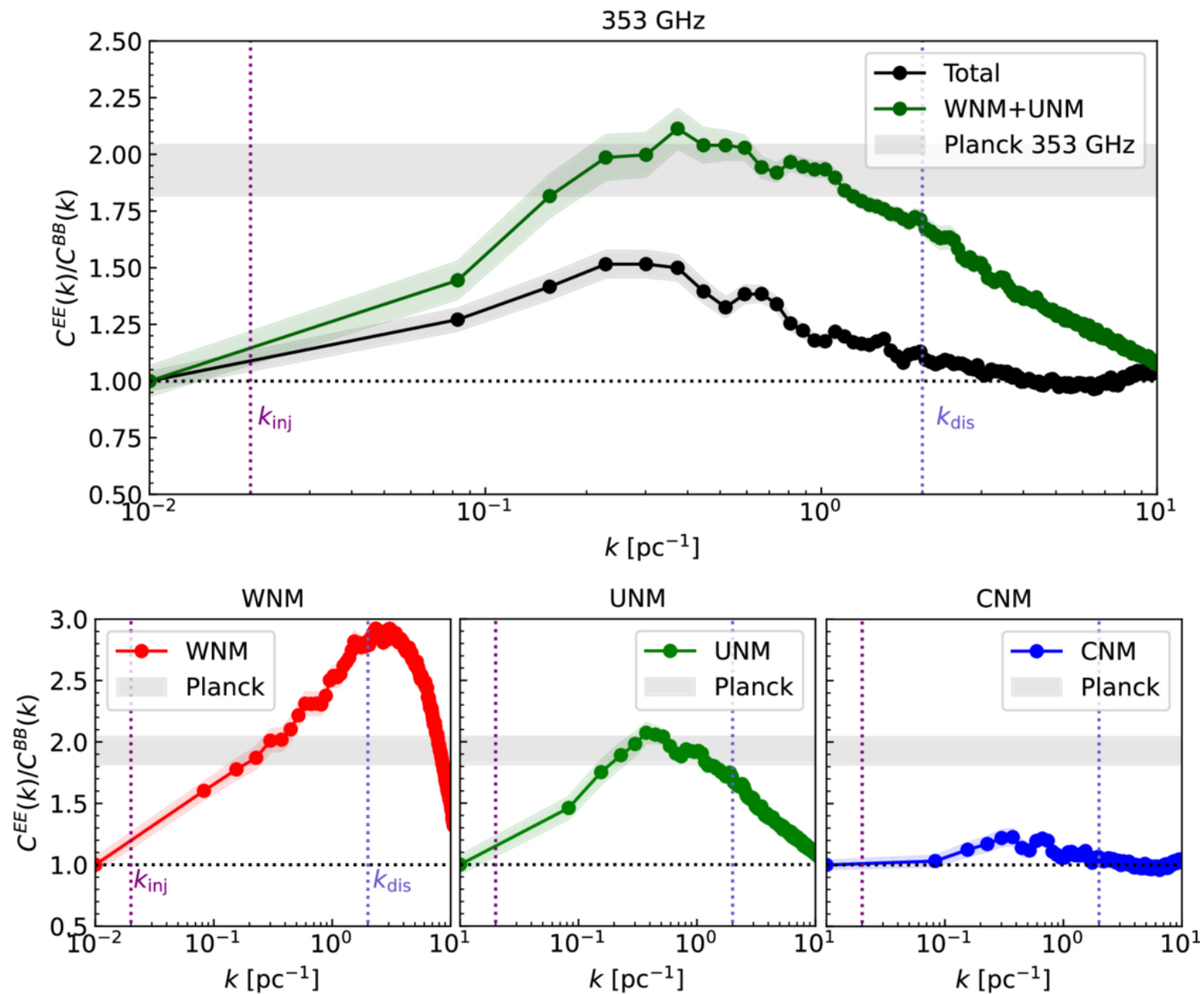
Figure 7. from Yue Hu et al 2026 Astrophys. J. 1007 doi:10.3847/1538-4357/ae8998 https://dx.doi.org/10.3847/1538-4357/ae8998 © 2026. The Author(s). Published by the American Astronomical Society.
