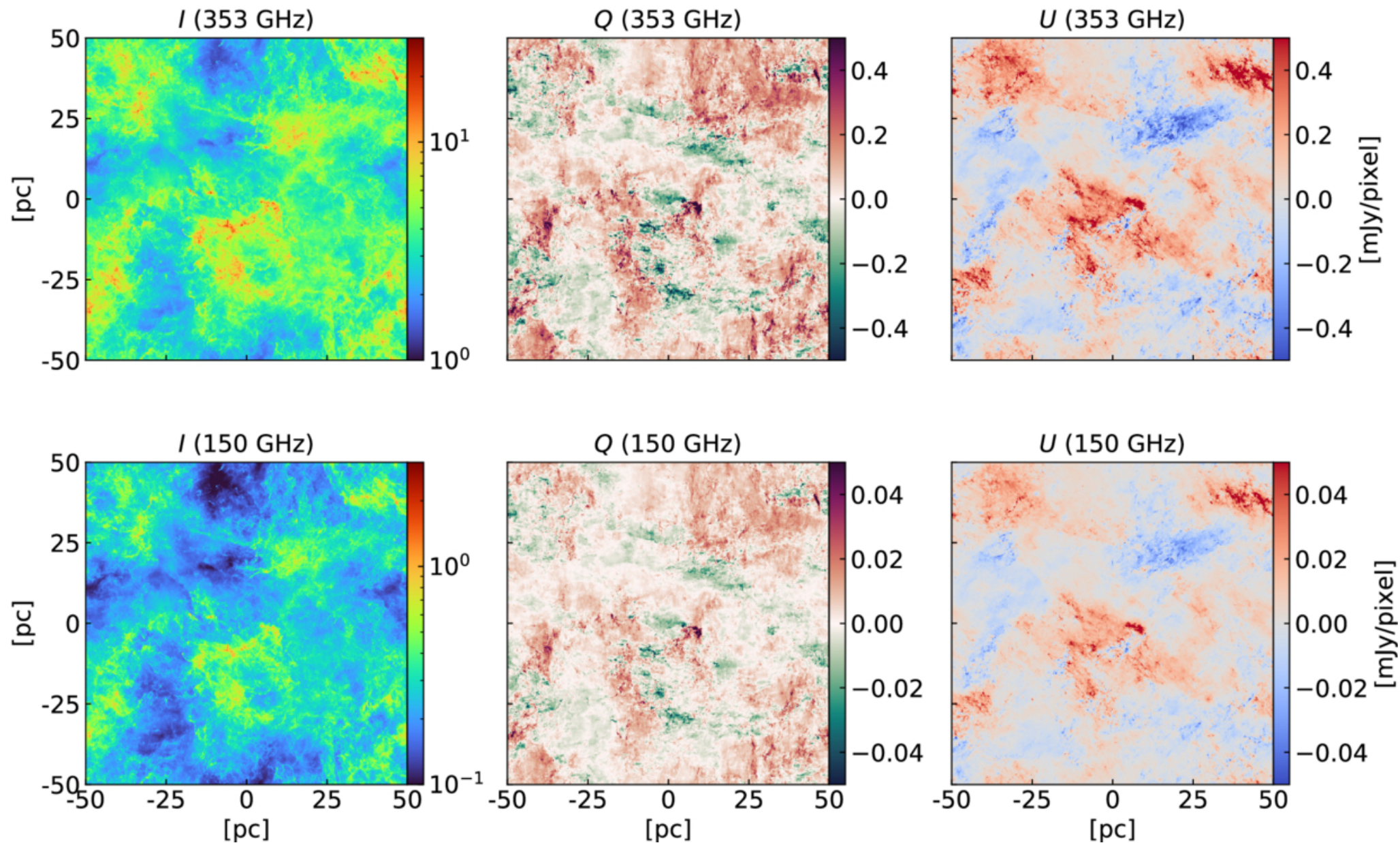
Figure 5. from Yue Hu et al 2026 Astrophys. J. 1007 doi:10.3847/1538-4357/ae8998 https://dx.doi.org/10.3847/1538-4357/ae8998 © 2026. The Author(s). Published by the American Astronomical Society.
