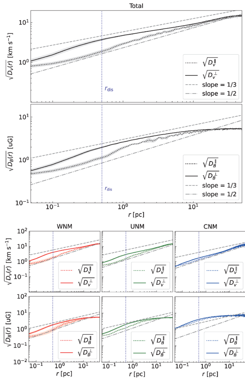
Figure 4. from Yue Hu et al 2026 Astrophys. J. 1007 doi:10.3847/1538-4357/ae8998 https://dx.doi.org/10.3847/1538-4357/ae8998 © 2026. The Author(s). Published by the American Astronomical Society.
