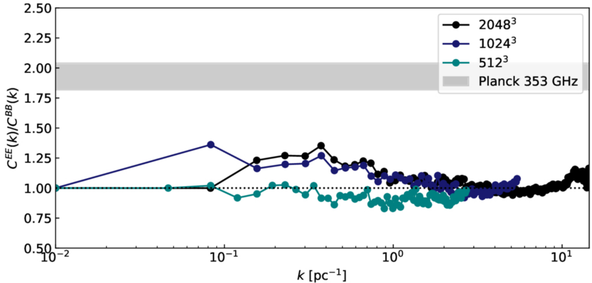
Figure 10. from Yue Hu et al 2026 Astrophys. J. 1007 doi:10.3847/1538-4357/ae8998 https://dx.doi.org/10.3847/1538-4357/ae8998 © 2026. The Author(s). Published by the American Astronomical Society.
