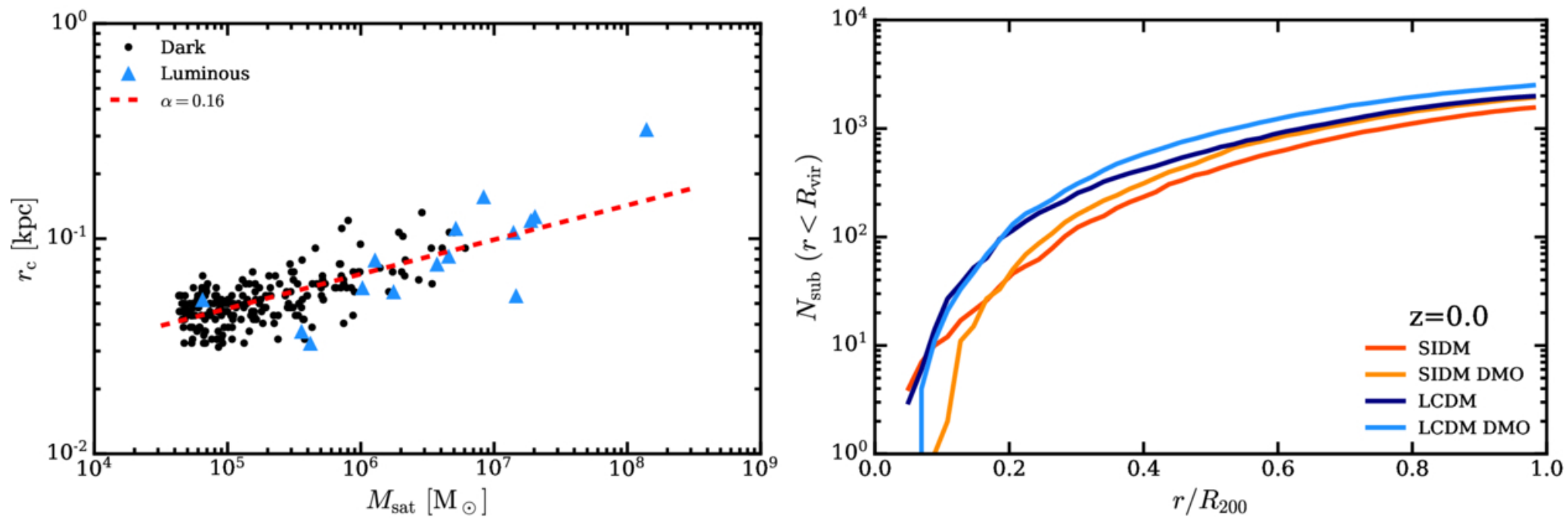
Figure 7. from Thales A. Gutcke et al 2026 Astrophys. J. 1007 doi:10.3847/1538-4357/ae879a https://dx.doi.org/10.3847/1538-4357/ae879a © 2026. The Author(s). Published by the American Astronomical Society.
