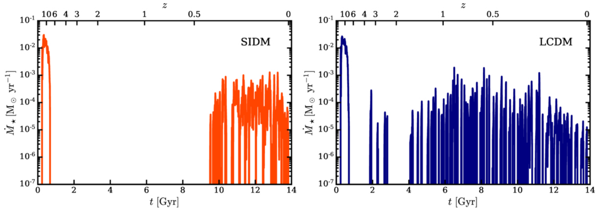
Figure 6. from Thales A. Gutcke et al 2026 Astrophys. J. 1007 doi:10.3847/1538-4357/ae879a https://dx.doi.org/10.3847/1538-4357/ae879a © 2026. The Author(s). Published by the American Astronomical Society.
