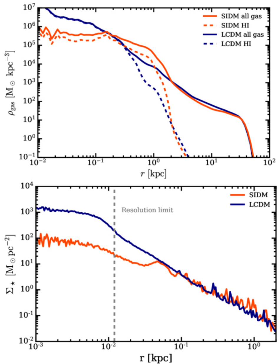
Figure 5. from Thales A. Gutcke et al 2026 Astrophys. J. 1007 doi:10.3847/1538-4357/ae879a https://dx.doi.org/10.3847/1538-4357/ae879a © 2026. The Author(s). Published by the American Astronomical Society.
