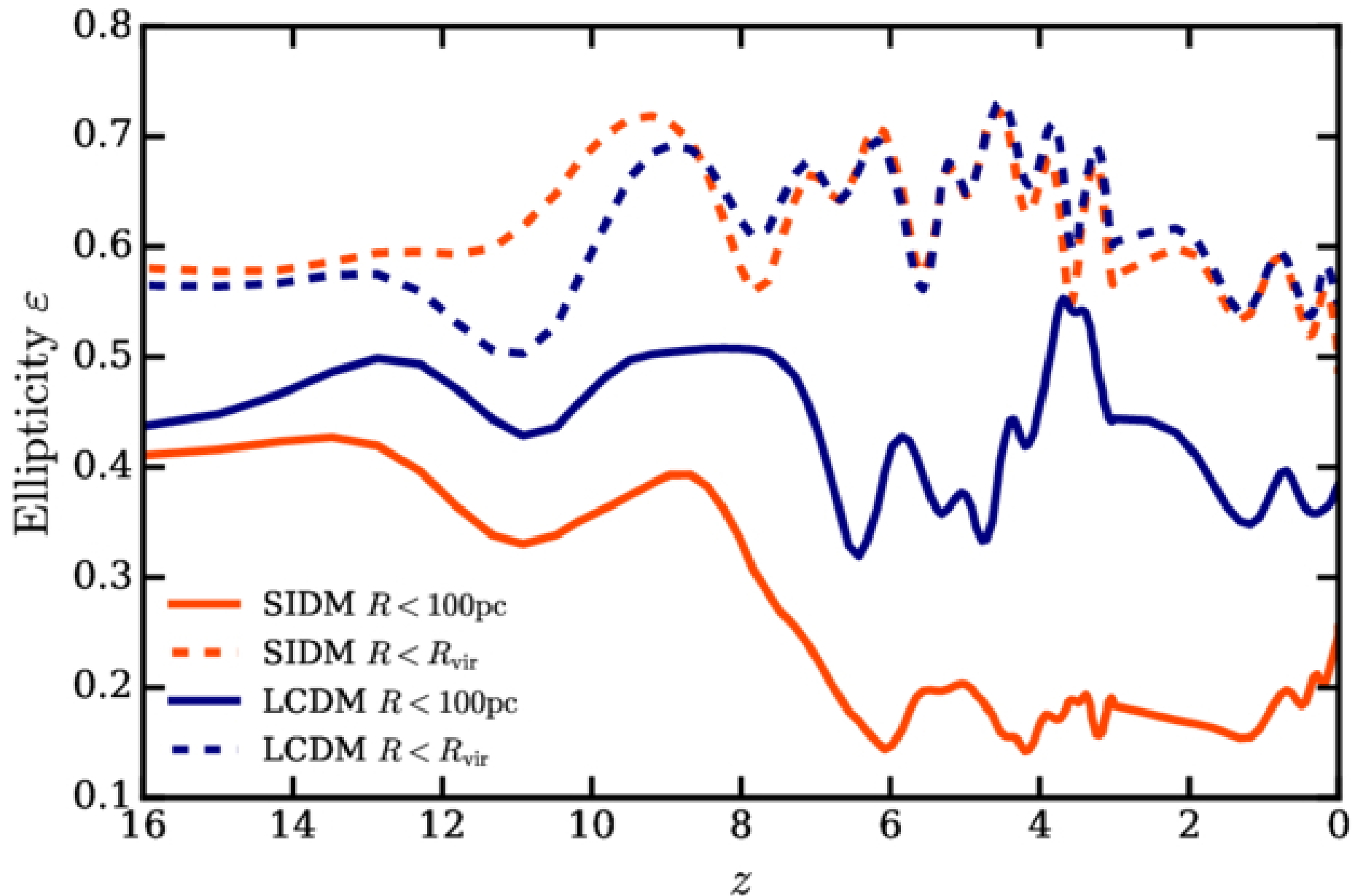
Figure 4. from Thales A. Gutcke et al 2026 Astrophys. J. 1007 doi:10.3847/1538-4357/ae879a https://dx.doi.org/10.3847/1538-4357/ae879a © 2026. The Author(s). Published by the American Astronomical Society.
