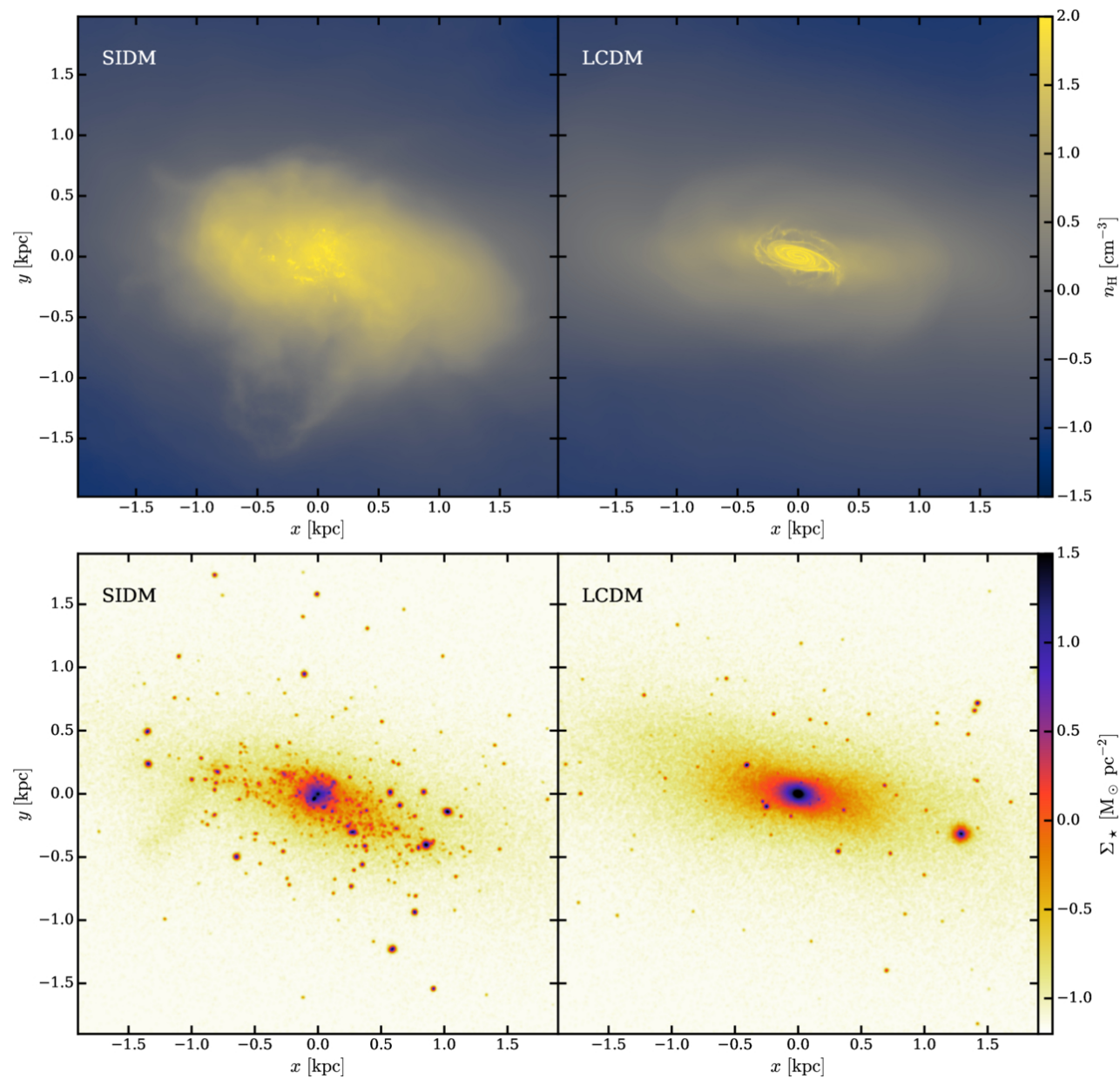
Figure 3. from Thales A. Gutcke et al 2026 Astrophys. J. 1007 doi:10.3847/1538-4357/ae879a https://dx.doi.org/10.3847/1538-4357/ae879a © 2026. The Author(s). Published by the American Astronomical Society.
