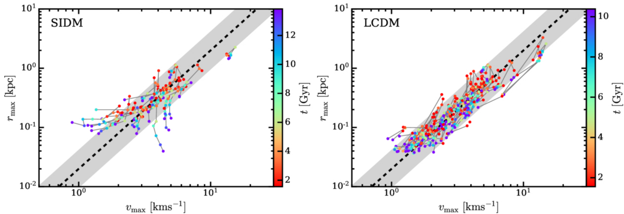
Figure 10. from Thales A. Gutcke et al 2026 Astrophys. J. 1007 doi:10.3847/1538-4357/ae879a https://dx.doi.org/10.3847/1538-4357/ae879a © 2026. The Author(s). Published by the American Astronomical Society.
