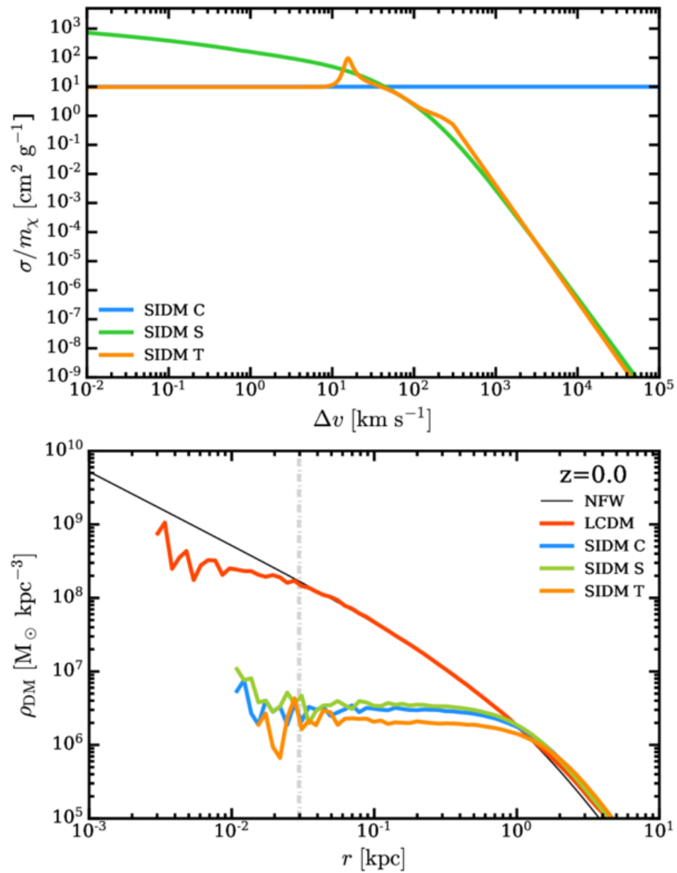
Figure 1. from Thales A. Gutcke et al 2026 Astrophys. J. 1007 doi:10.3847/1538-4357/ae879a https://dx.doi.org/10.3847/1538-4357/ae879a © 2026. The Author(s). Published by the American Astronomical Society.
