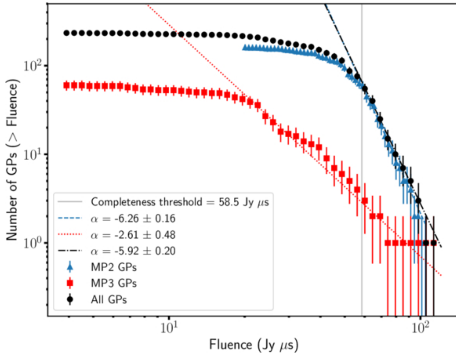
Figure 6. from Saptarshi Sarkar et al 2026 Astrophys. J. 1007 doi:10.3847/1538-4357/ae8798 https://dx.doi.org/10.3847/1538-4357/ae8798 © 2026. The Author(s). Published by the American Astronomical Society.
