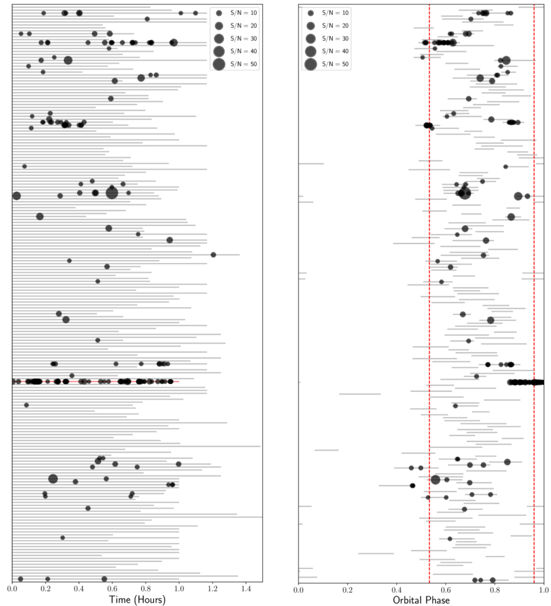
Figure 4. from Saptarshi Sarkar et al 2026 Astrophys. J. 1007 doi:10.3847/1538-4357/ae8798 https://dx.doi.org/10.3847/1538-4357/ae8798 © 2026. The Author(s). Published by the American Astronomical Society.
