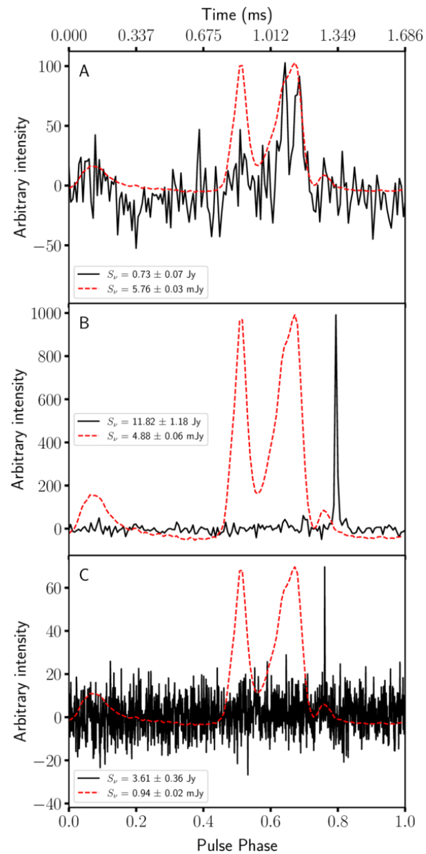
Figure 3. from Saptarshi Sarkar et al 2026 Astrophys. J. 1007 doi:10.3847/1538-4357/ae8798 https://dx.doi.org/10.3847/1538-4357/ae8798 © 2026. The Author(s). Published by the American Astronomical Society.
