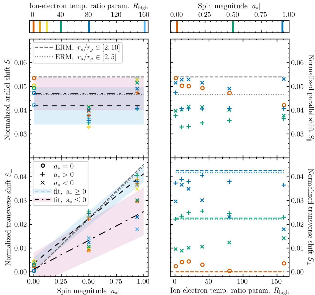
Figure 4. from Delilah E. A. Gates et al 2026 Astrophys. J. 1007 doi:10.3847/1538-4357/ae8787 https://dx.doi.org/10.3847/1538-4357/ae8787 © 2026. The Author(s). Published by the American Astronomical Society.
