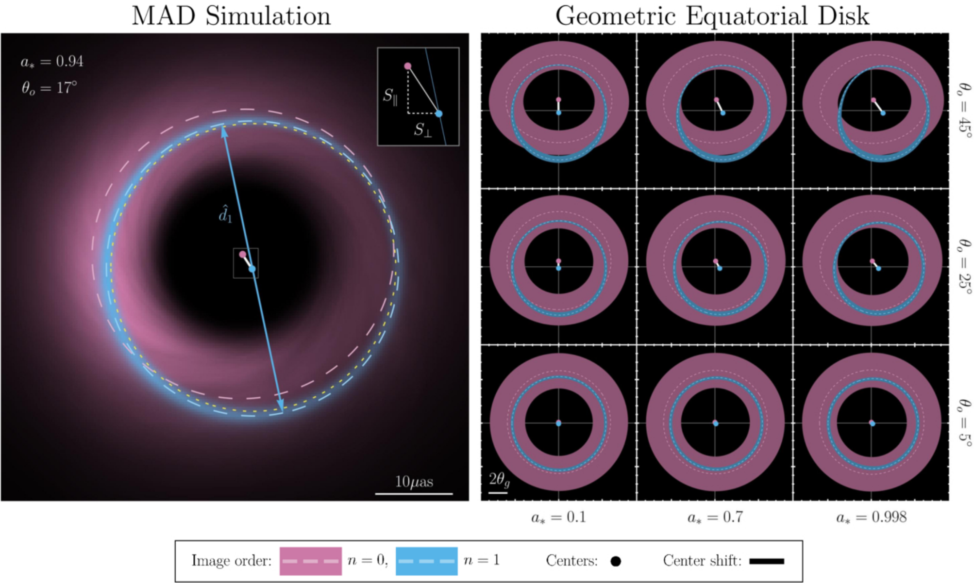
Figure 1. from Delilah E. A. Gates et al 2026 Astrophys. J. 1007 doi:10.3847/1538-4357/ae8787 https://dx.doi.org/10.3847/1538-4357/ae8787 © 2026. The Author(s). Published by the American Astronomical Society.
