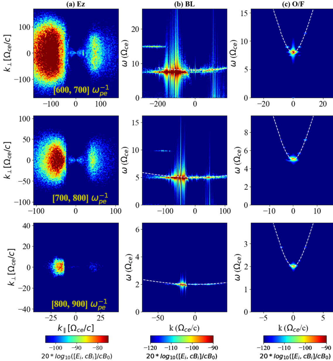
Figure 4. from Mehdi Yousefzadeh et al 2026 Astrophys. J. 1007 doi:10.3847/1538-4357/ae8771 https://dx.doi.org/10.3847/1538-4357/ae8771 © 2026. The Author(s). Published by the American Astronomical Society.
